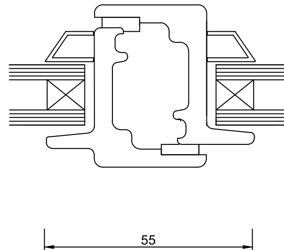
Meeting Rail
