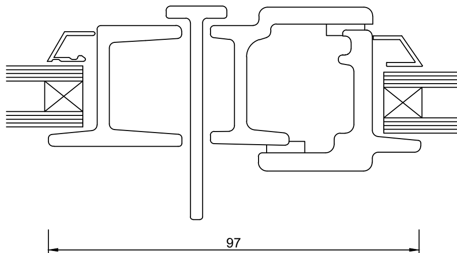
Coupling Detail
